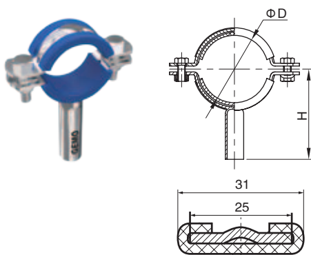
TH6-B Tubing Hanger
