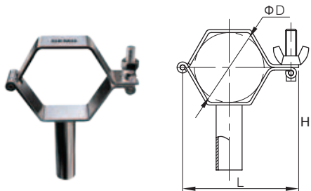
TH3-C Tubing Hanger
