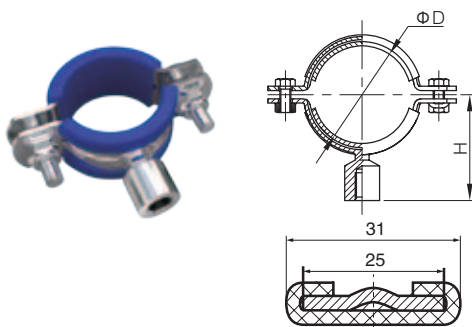
TH6-B Tubing Hanger
