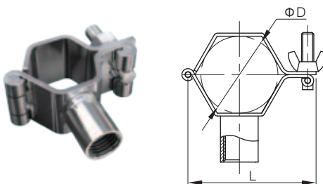
TH3-B Tubing Hanger
